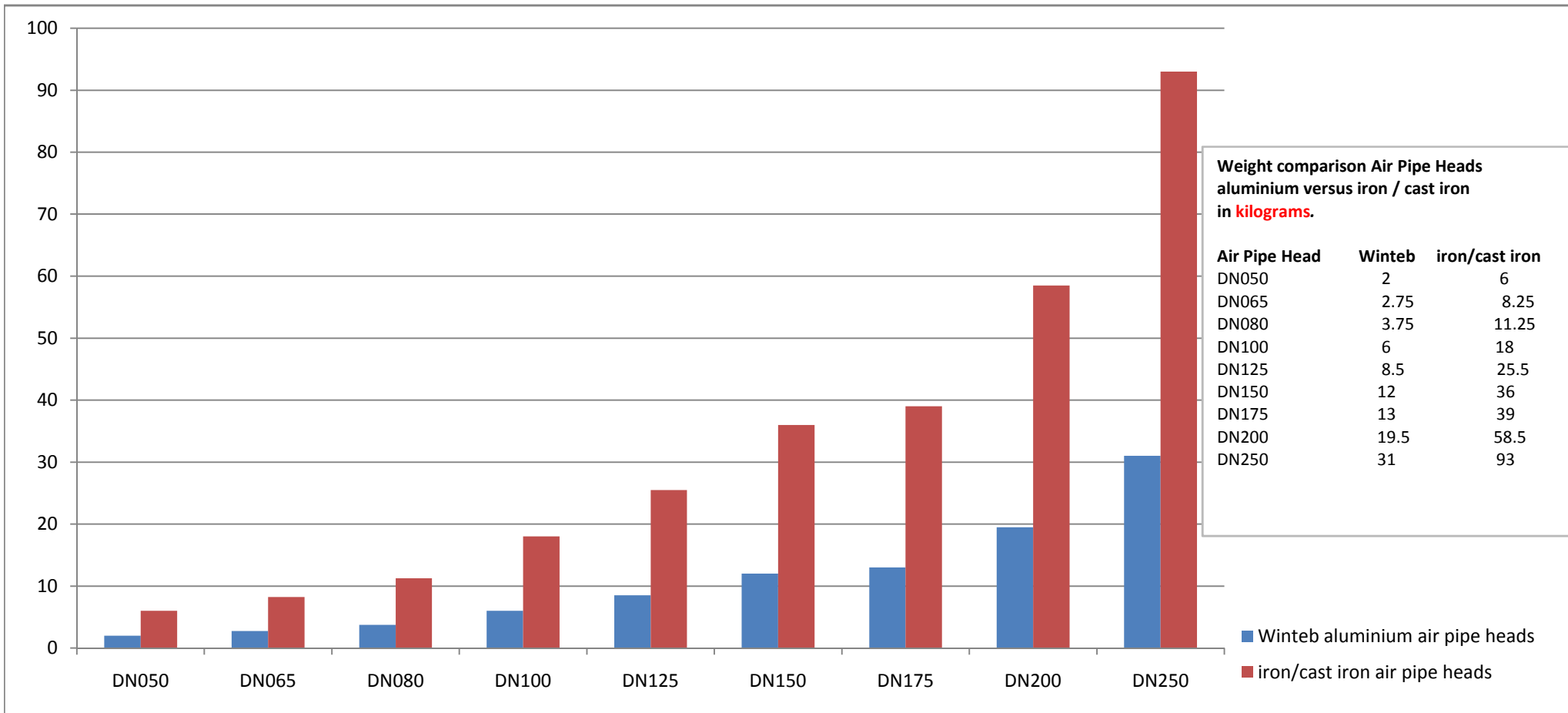
Weight comparison Air Pipe Heads Winteb aluminium versus iron/cast iron in kilograms
